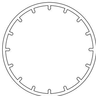
503.24115 Round 44x3.5 wheel + crown
