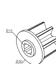
575.12150
