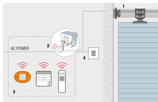
1. TUBULAR MOTOR 2. MINIATURISED TAG TT2N SERIES CONTROL UNIT CONNECTED VIA MAINS POWER SUPPLY 3. TRANSMITTER 4. PUSHBUTTON
