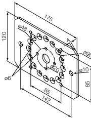
525.10089 175x120 support for sides
