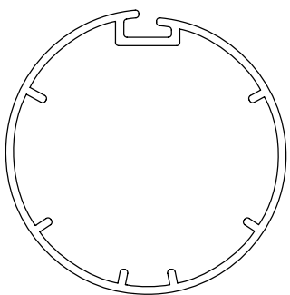
513.24215 Round 44 wheel + crown
