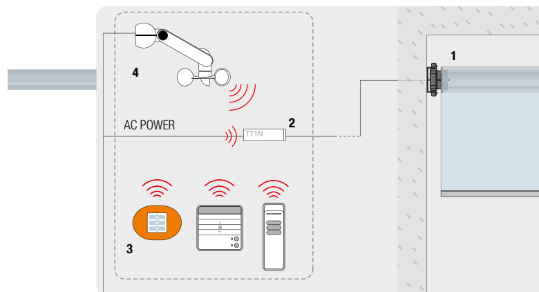
1. TUBULAR MOTOR 2. TAG TT1N SERIES CONTROL UNIT 3. TRANSMITTER 4. NEMO SERIES RADIO-CONTROLLED ANEMOMETER
