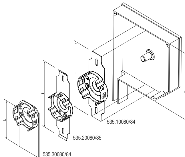
Application example
