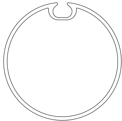
503.15301 Notch 53x2 wheel + crown
