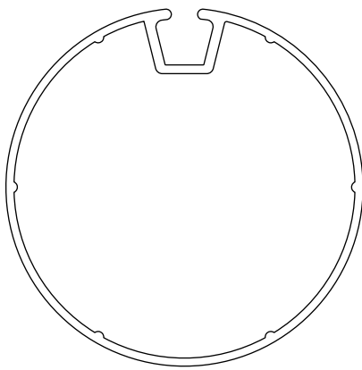
503.15300 Notch 53x1.5 wheel + crown
