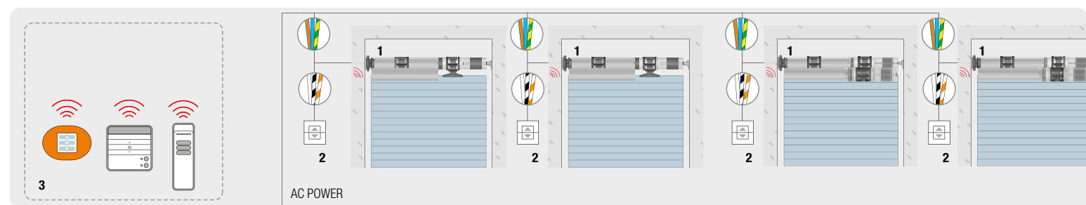
1. TUBULAR MOTOR 2. INDIVIDUAL "UP/DOWN" BUTTON CONNECTED TO TTBus** 3. TRANSMITTER FOR SINGLE OR GROUP CONTROL
