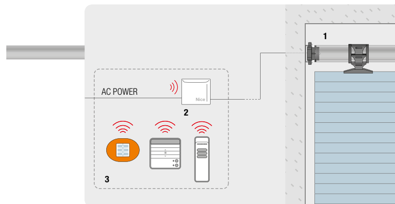
1. TUBULAR MOTOR 2. MINDY TT4 SERIES CONTROL UNIT 3. TRANSMITTER
