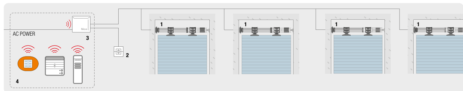
1. TUBULAR MOTOR 2. GROUP "UP/DOWN" BUTTON 3. MINDY TT4* SERIES "UP/DOWN" CONTROL UNIT 4. TRANSMITTER FOR GROUP CONTROL
