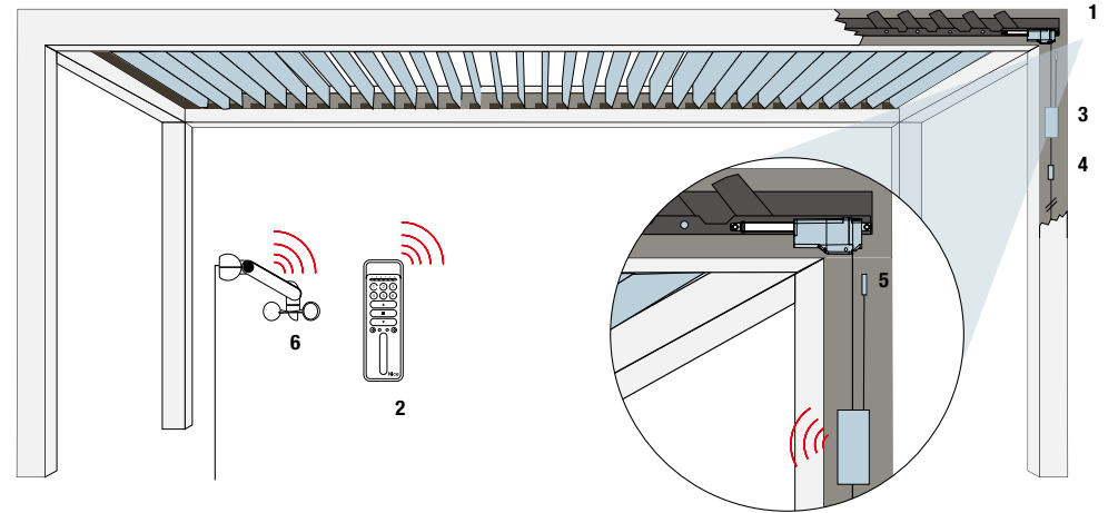
1. Motor 2. Transmitter 3. Control unit 4. Power Supply module 5. Temperature Sensor 6. Climatic sensor
