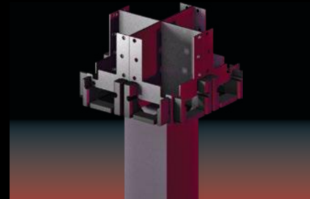
4-Module-Connector
