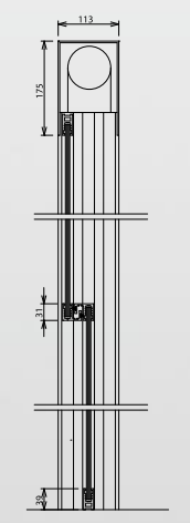
Type 2 Motorized
