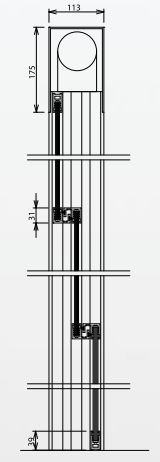
Type 2 Motorized
