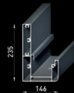
Integrated Beam
